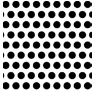
R60 05035 35% open area 5.0mm round x 8.4mm pitch
