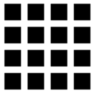
SH90 08048 48% open area 8mm x 8mm Square 90° pitch
