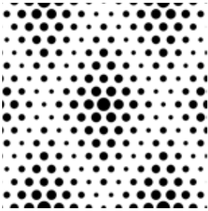
P1 Diamond 50% open area 8, 12, 16, 19 & 25mm hole x 26.8mm pitch
