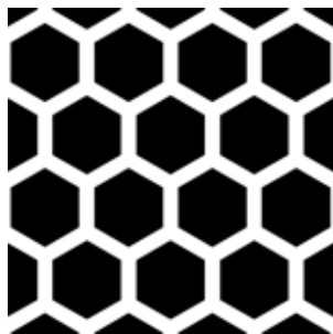
H60 95064 64% open area 9.5mm x 11.9mm 60° stagger pitch
