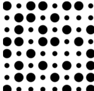
P1 Braille 26% open area 10 & 19mm x 35.9mm Braille pitch
