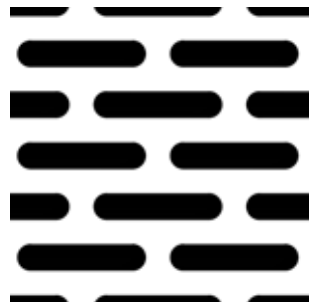
RS 25040 SST 40% open area 25mm x 5mm Single Stagger
